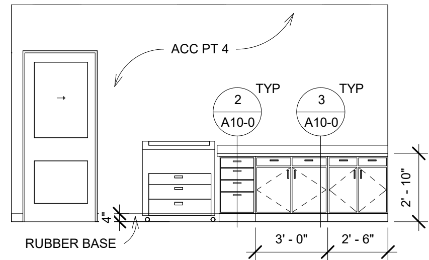
74 RECEPTION EAST 1/4" = 1'-0"
