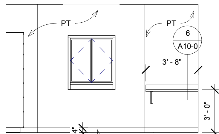
118 DRIVE-THRU WEST 1/4" = 1'-0"
