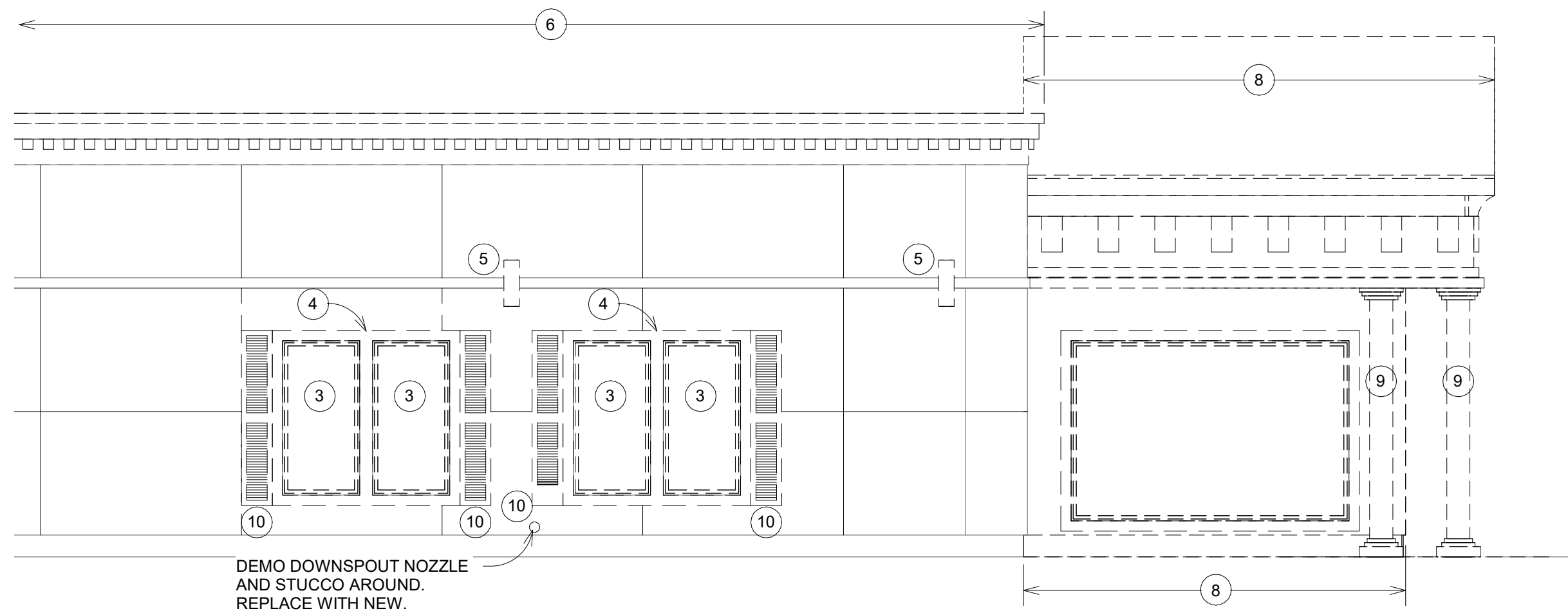
2 EAST DEMO ELEVATION - Callout 2 1/4" = 1'-0"
