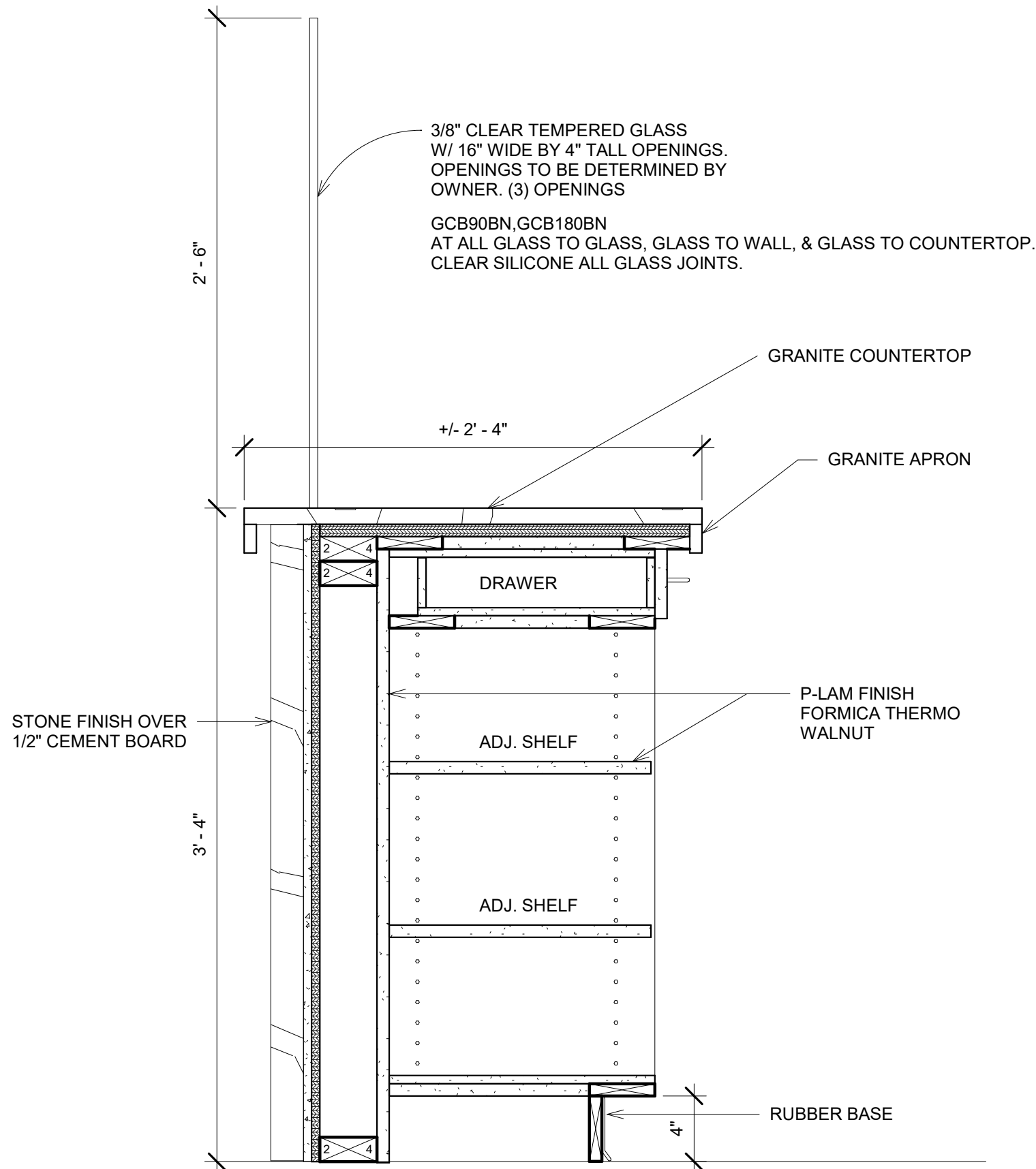
② PHARMACY CASEWORK 2 1 1/2" = 1'-0"
