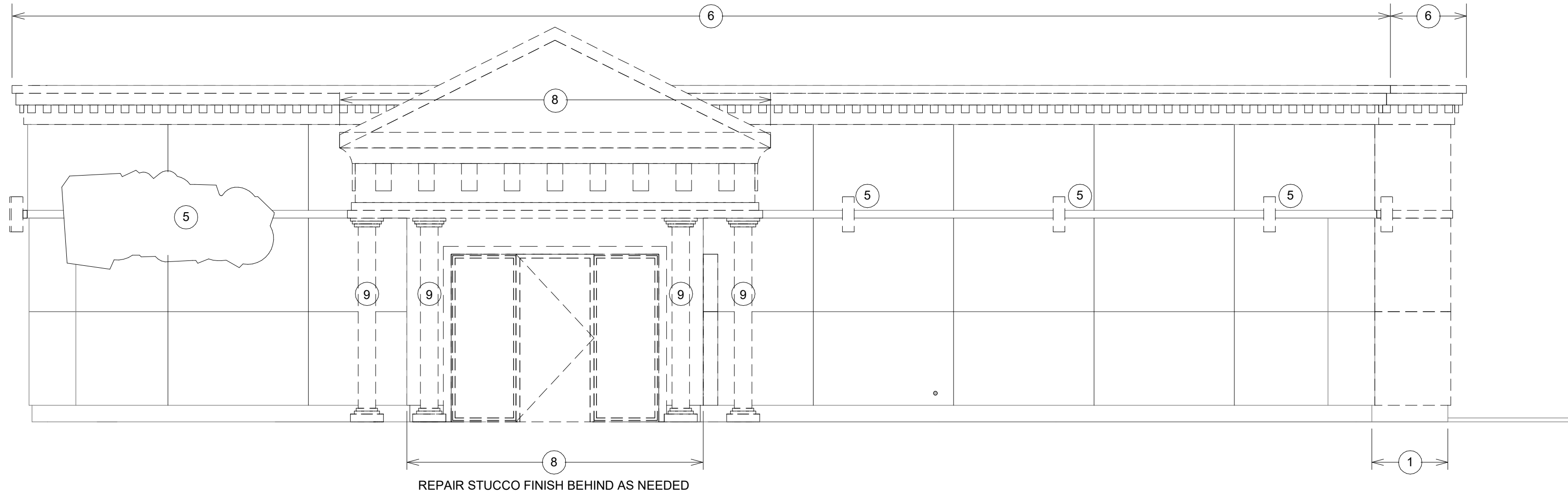
1 NORTH DEMO ELEVATION 1/4" = 1'-0"
