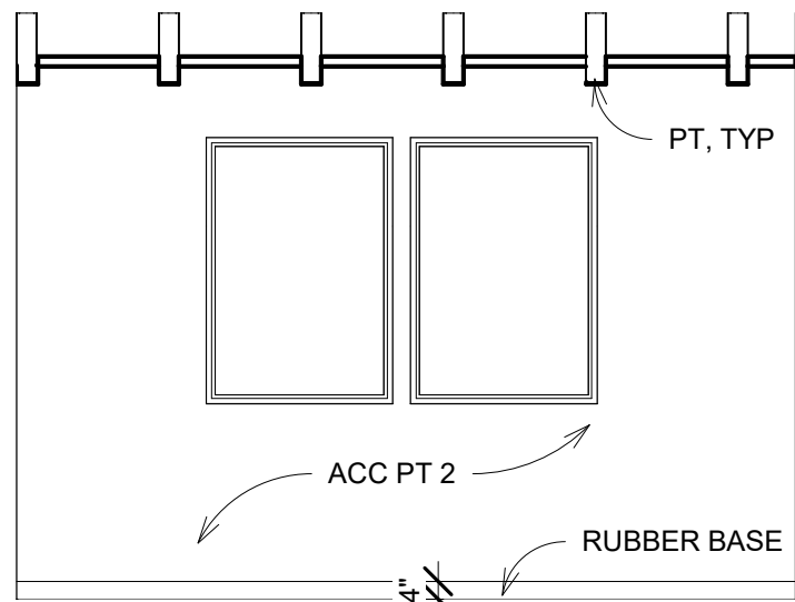
101 OFFICE 2 EAST 1/4" = 1'-0"
