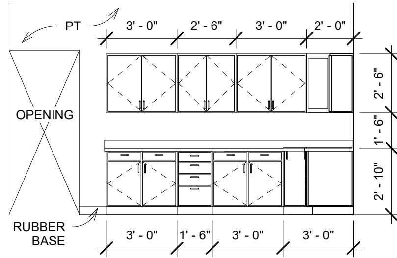
36 LAB WEST 1/4" = 1'-0"
