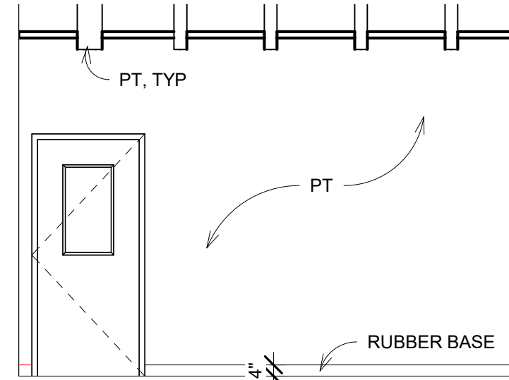
66 OFFICE 1 WEST 1/4" = 1'-0"
