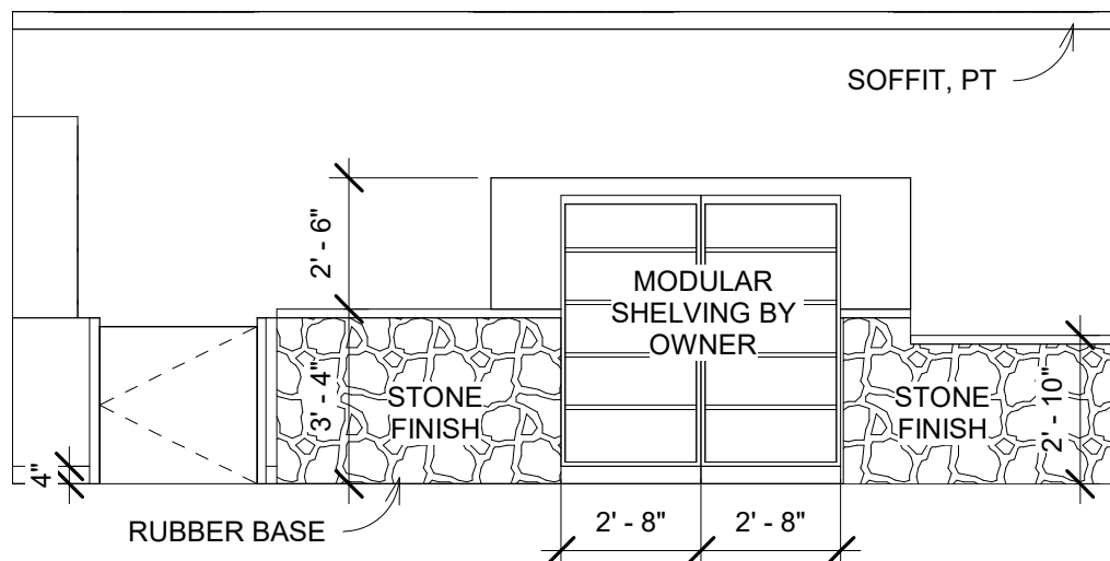
107 PHARMACY WAIT SOUTH 2 1/4" = 1'-0"
