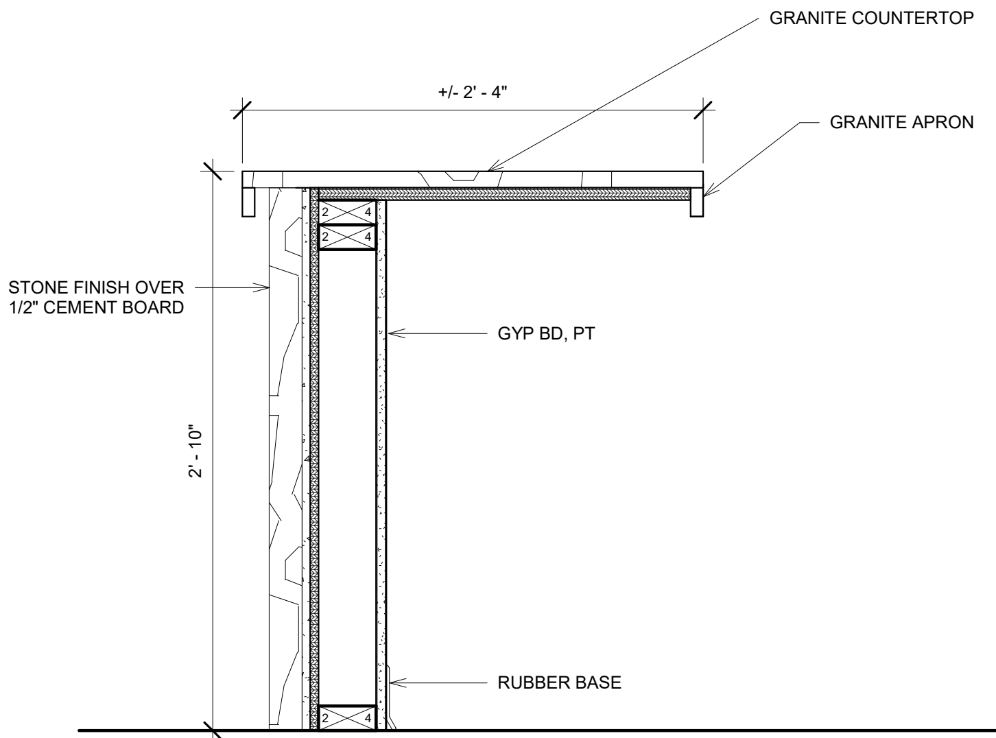
① PHARMACY CASEWORK 1 1 1/2" = 1'-0"
