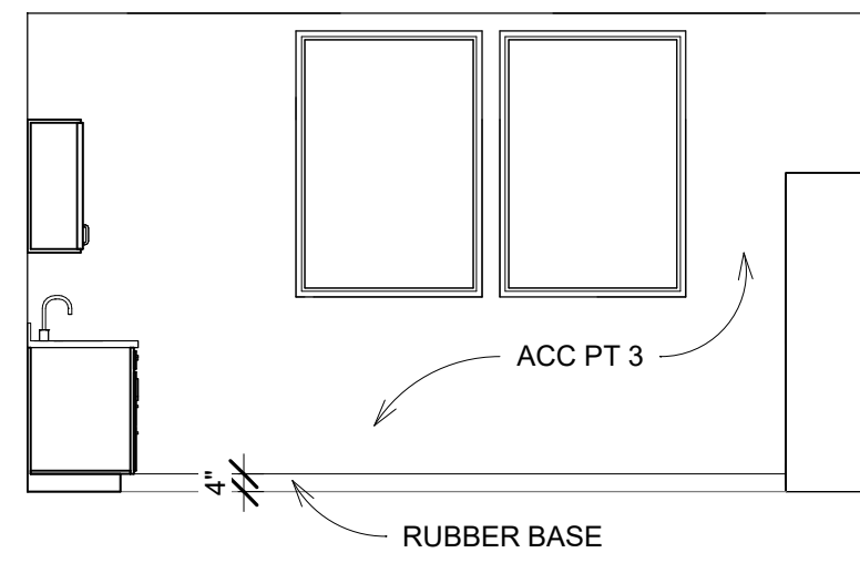
97 BREAKROOM EAST 1/4" = 1'-0"
