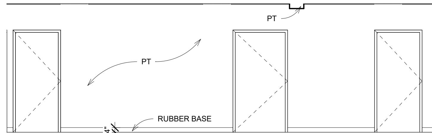
89 CORR 8 WEST 1/4" = 1'-0"
