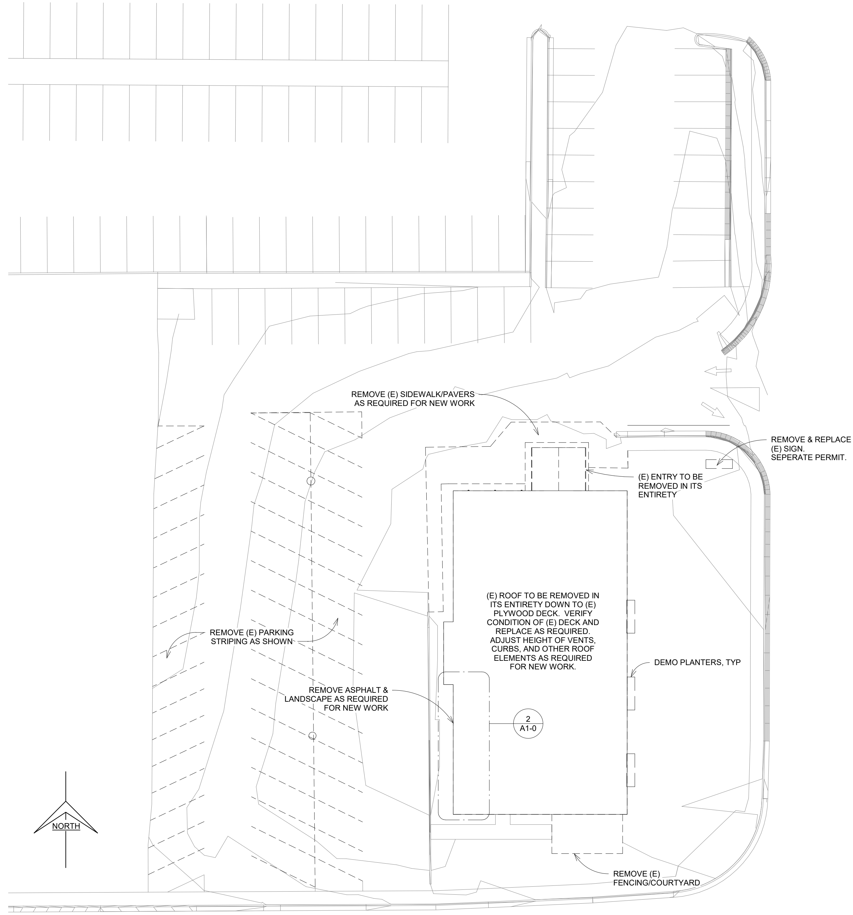
1 DEMO SITE PLAN 1" = 20'-0"
