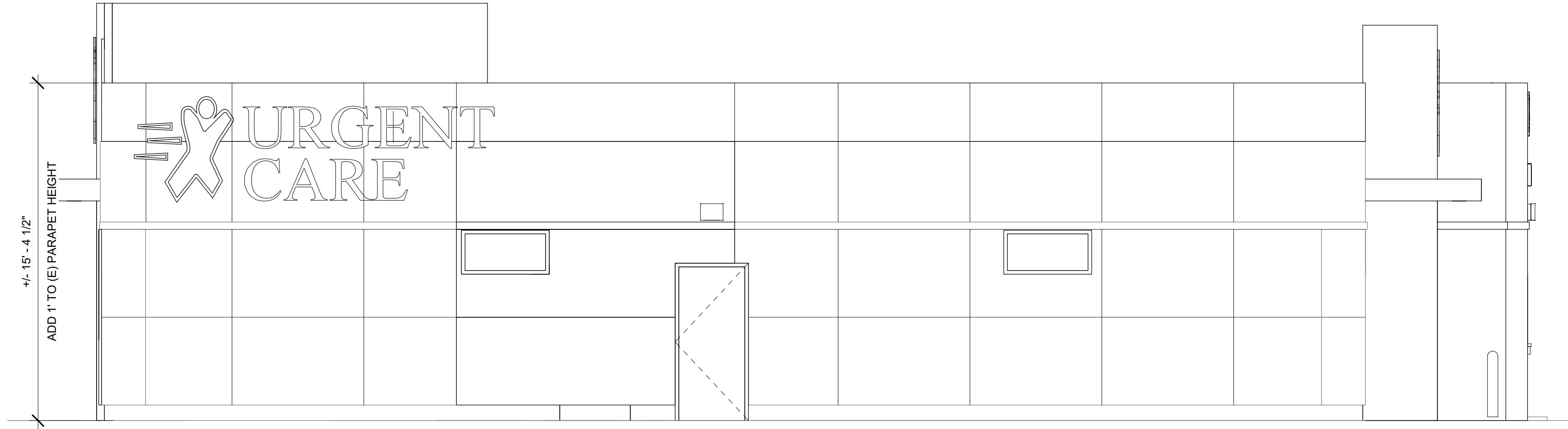
① NEW NORTH 1/4" = 1'-0"
