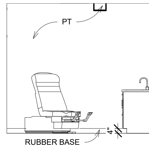
45 EXAM 5 EAST 1/4" = 1'-0"
