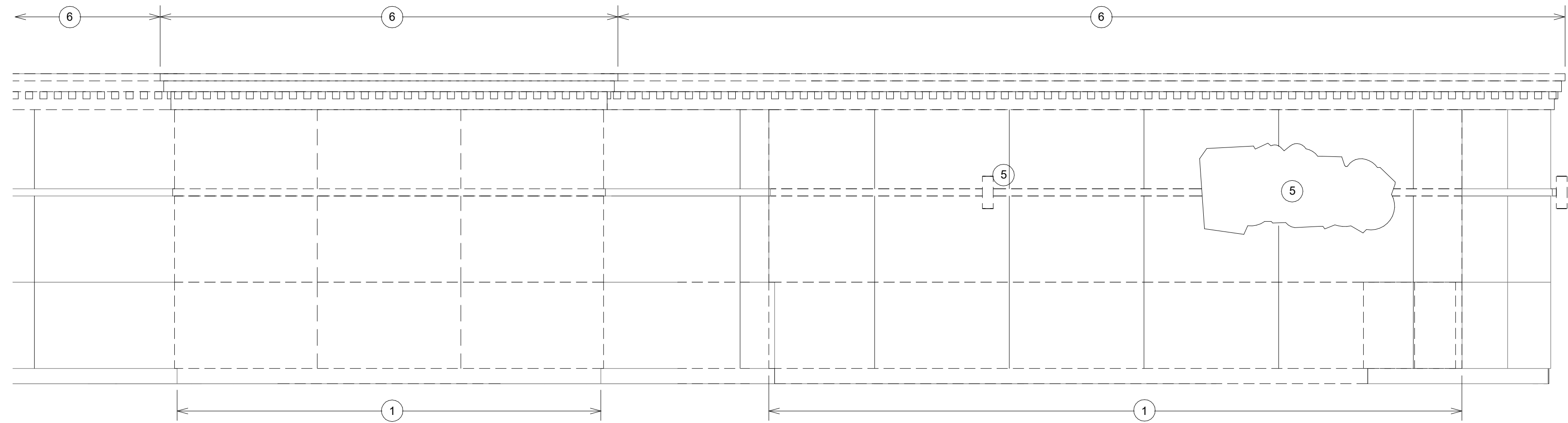
3 WEST DEMO ELEVATION - Callout 2 1/4" = 1'-0"
