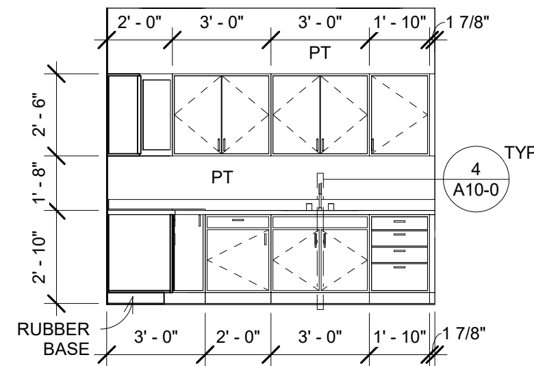
96 BREAKROOM NORTH 1/4" = 1'-0"
