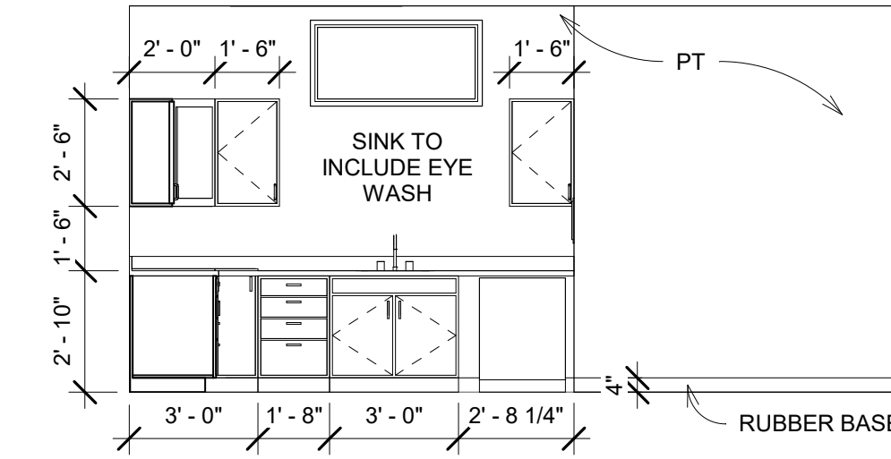
33 LAB NORTH 1/4" = 1'-0"
