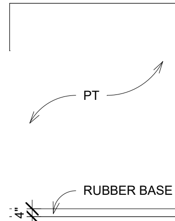
31 STORAGE SOUTH 1/4" = 1'-0"
