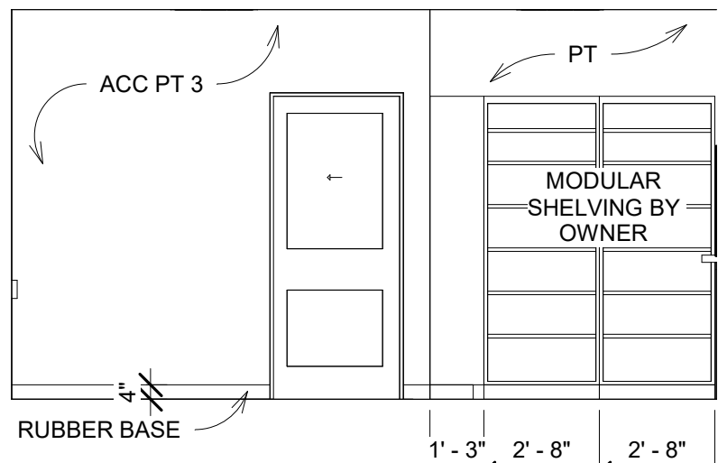
109 PHARMACY WAIT EAST 1/4" = 1'-0"
