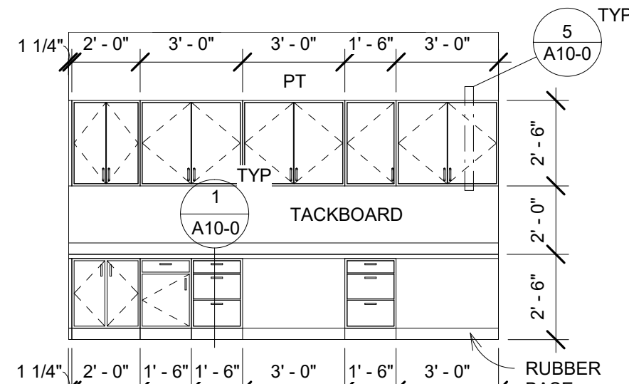
70 PROVIDERS EAST 1/4" = 1'-0"
