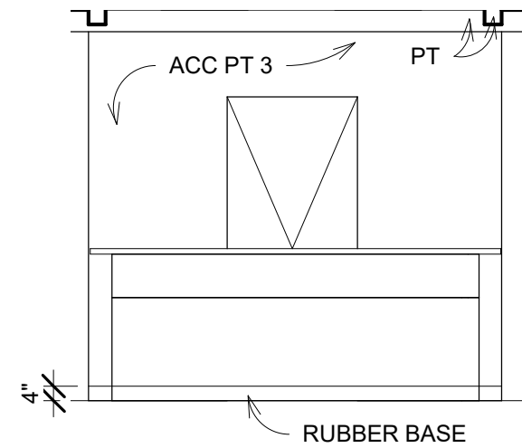
49 CORR 6 SOUTH 1/4" = 1'-0"
