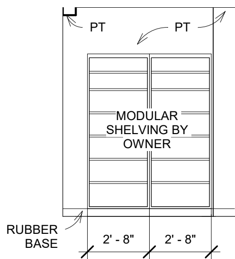
119 DRIVE-THRU SOUTH 1/4" = 1'-0"
