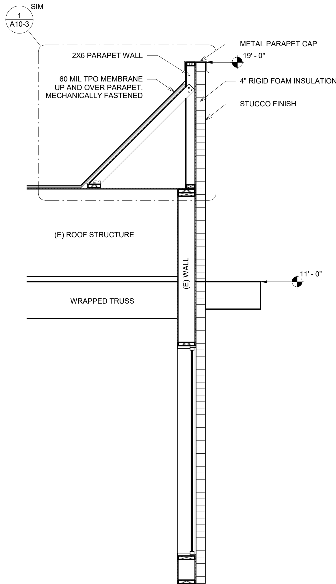
2 Wall Section 2 1/2" = 1'-0"
