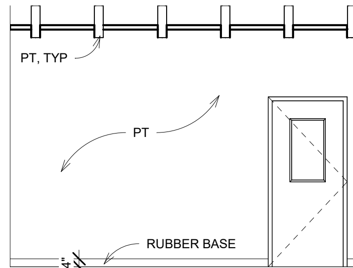
103 OFFICE 2 WEST 1/4" = 1'-0"
