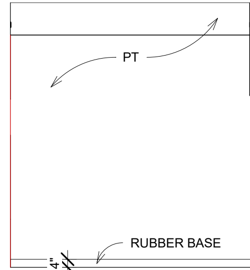
65 OFFICE 1 SOUTH 1/4" = 1'-0"
