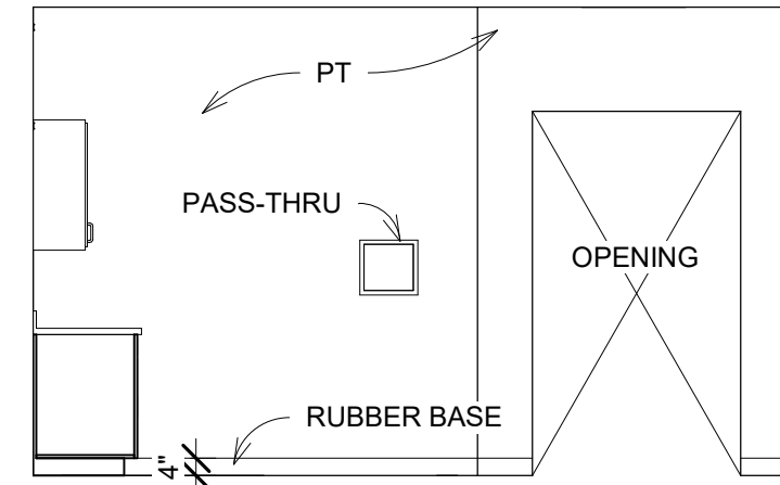
34 LAB EAST 1/4" = 1'-0"
