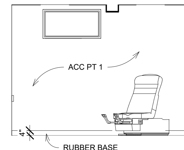
56 EXAM 6 EAST 1/4" = 1'-0"
