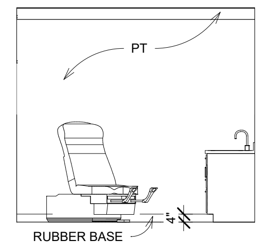
57 EXAM 6 SOUTH 1/4" = 1'-0"
