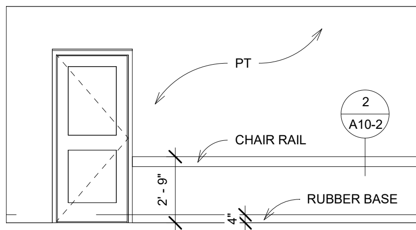
104 PHARMACY WAIT NORTH 1 1/4" = 1'-0"
