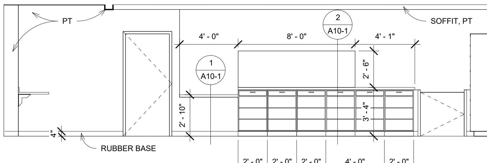
122 PHARMACY NORTH 1/4" = 1'-0"
