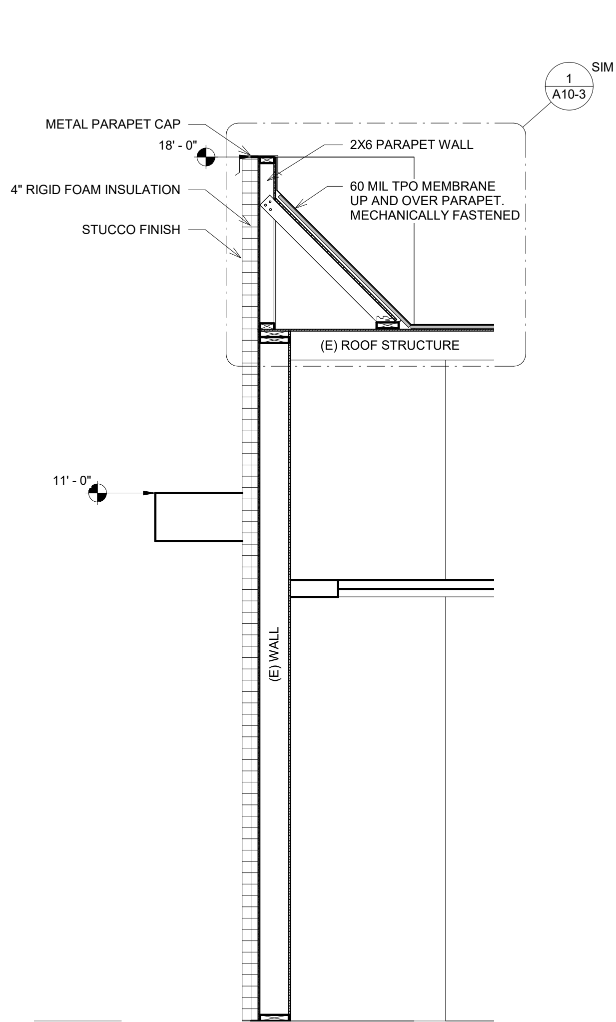
1 Wall Section 1 1/2" = 1'-0"
