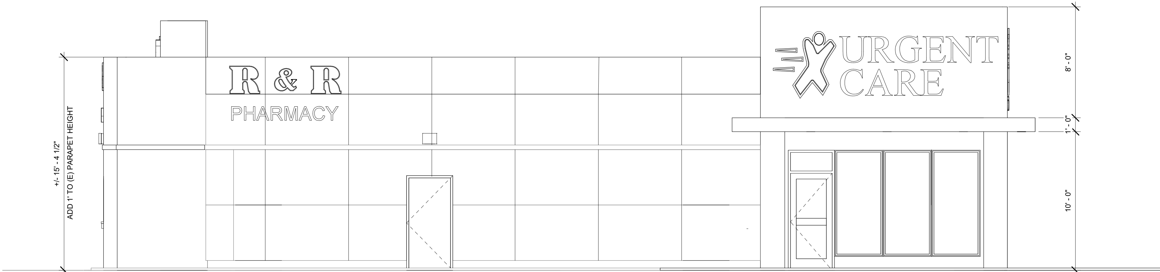
② NEW SOUTH 1/4" = 1'-0"
