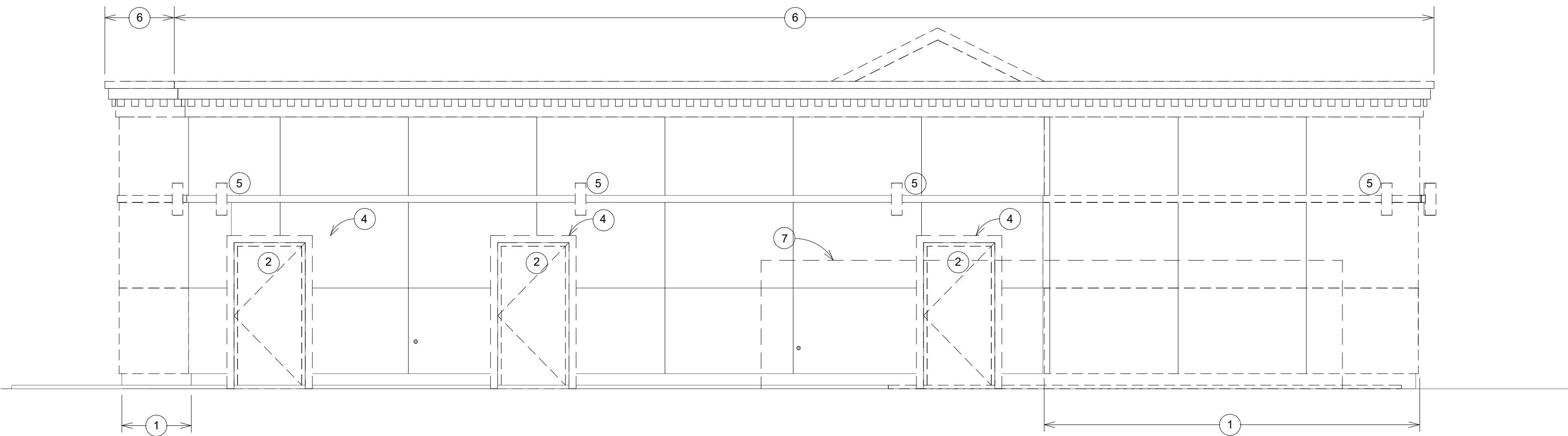
2 SOUTH DEMO ELEVATION 1/4" = 1'-0"
