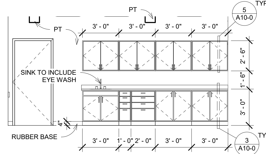
54 PROCEDURE WEST 1/4" = 1'-0"
