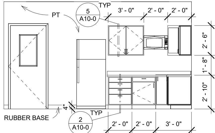
99 BREAKROOM WEST 1/4" = 1'-0"
