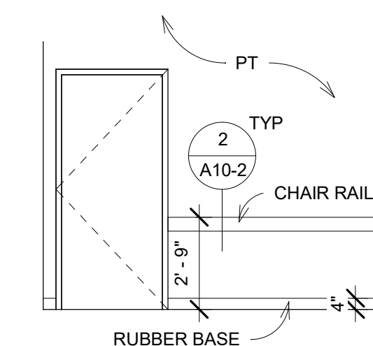
47 EXAM 5 WEST 1/4" = 1'-0"
