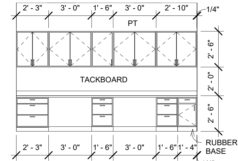
72 PROVIDERS WEST 1/4" = 1'-0"
