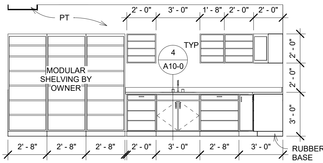
121 PHARMACY EAST 1/4" = 1'-0"
