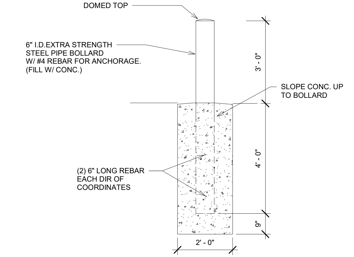
1 BOLLARD DETAIL 1/2" = 1'-0"
