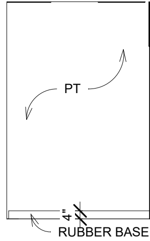
123 STORAGE 2 NORTH 1/4" = 1'-0"
