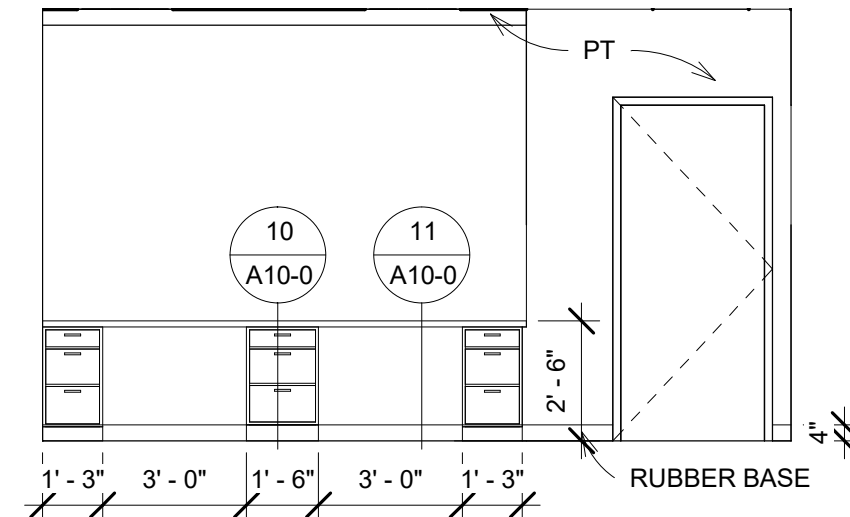
76 RECEPTION WEST 1/4" = 1'-0"
