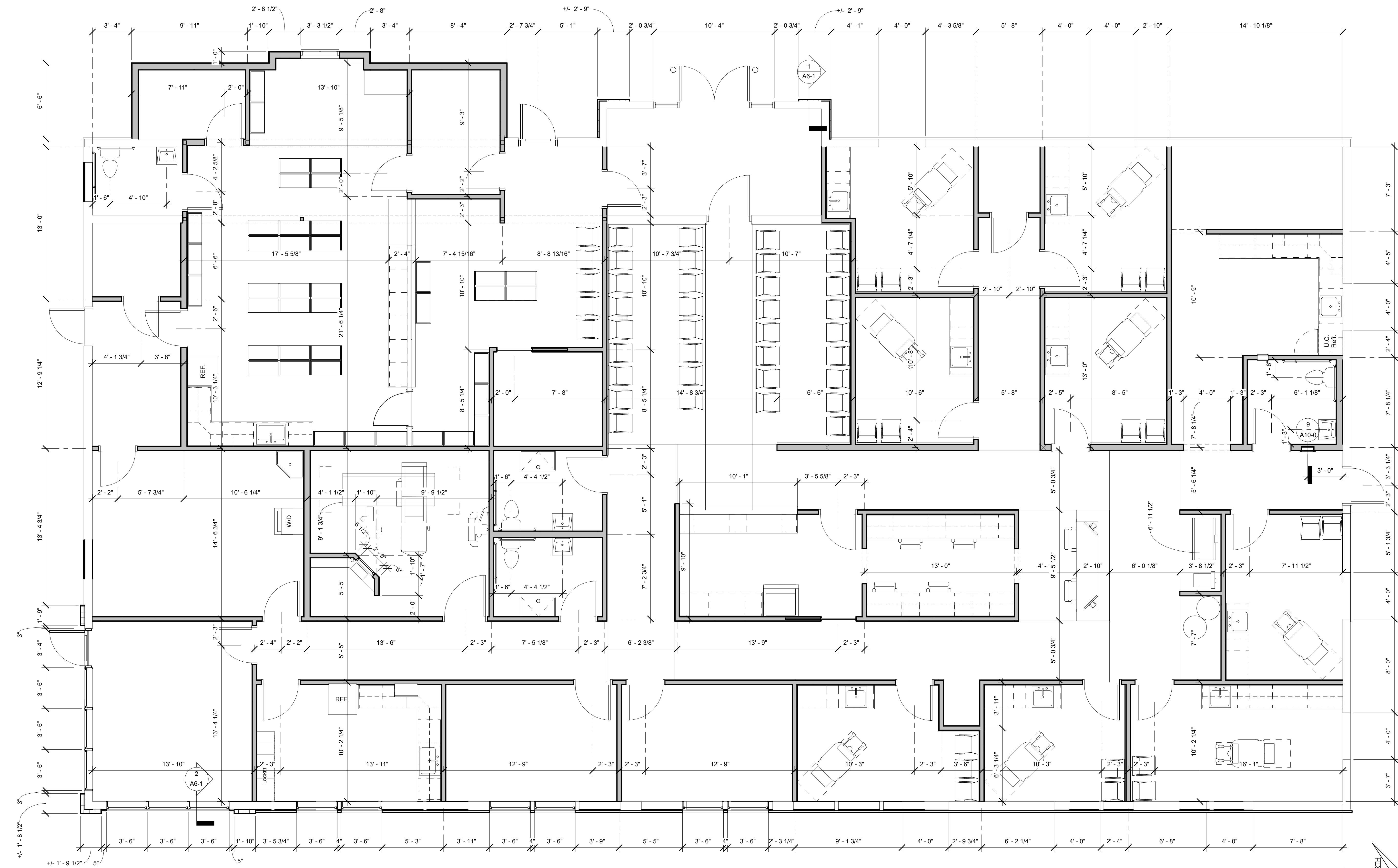
1 DIM NEW FLOOR PLAN 1/4" = 1'-0"
