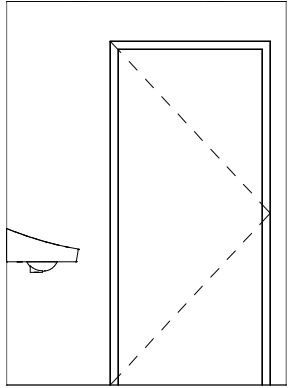
127 RR NORTH 1/4" = 1'-0"
