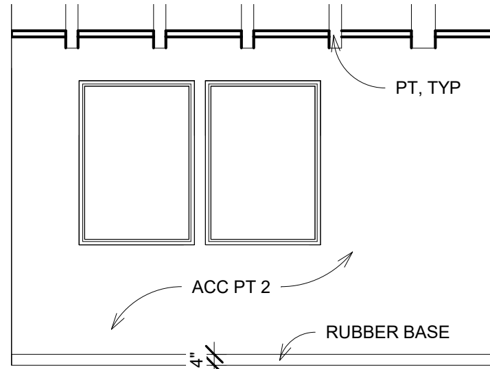
64 OFFICE 1 EAST 1/4" = 1'-0"
