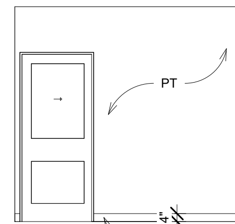
113 OFFICE WEST 1/4" = 1'-0"
