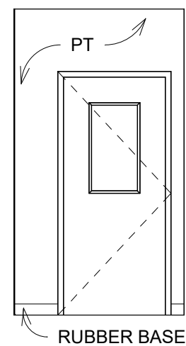
90 CORR 8 SOUTH 1/4" = 1'-0"
