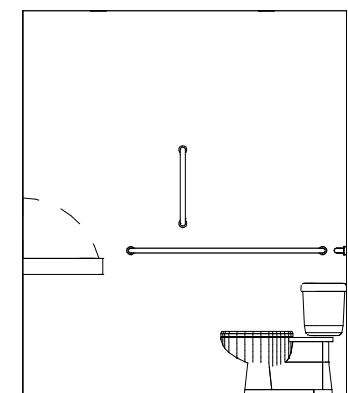
83 RR 3 SOUTH 1/4" = 1'-0"
