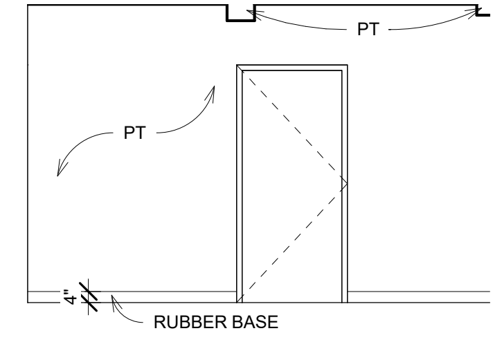
43 CORR 5 EAST 1/4" = 1'-0"
