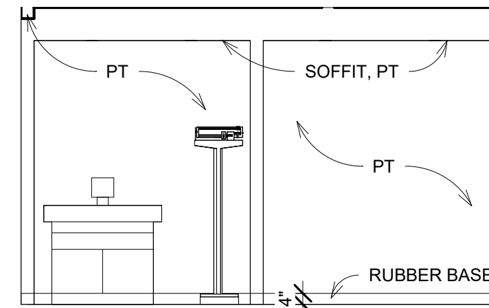
48 CORR 6 NORTH 1/4" = 1'-0"
