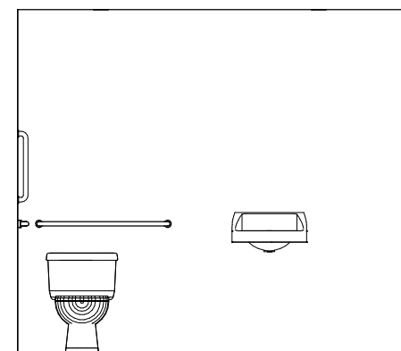
84 RR 3 WEST 1/4" = 1'-0"
