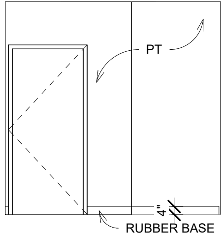
124 STORAGE 2 EAST 1/4" = 1'-0"
