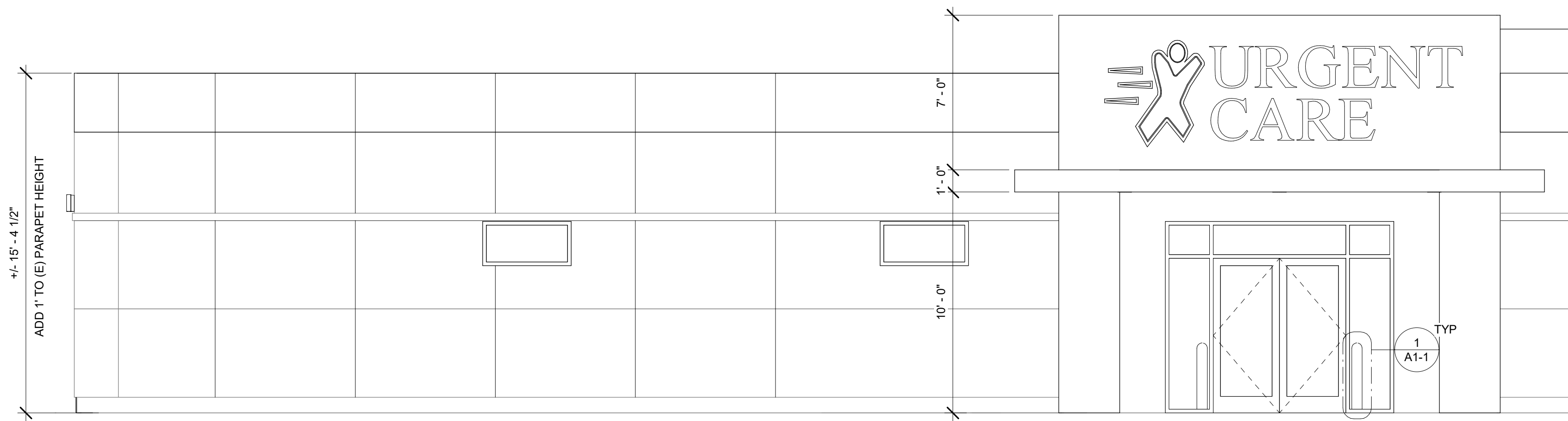
2 NEW WEST - Callout 1 1/4" = 1'-0"
