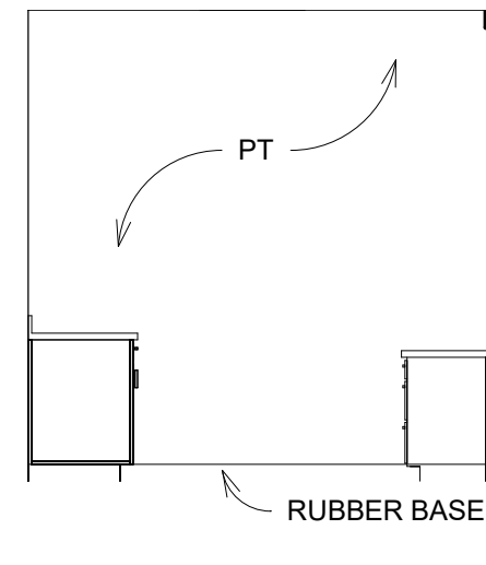
75 RECEPTION SOUTH 1/4" = 1'-0"
