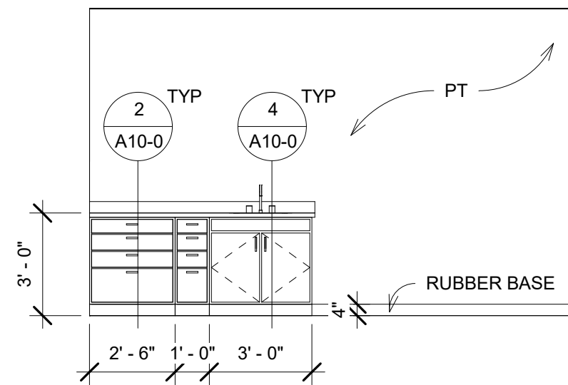
46 EXAM 5 SOUTH 1/4" = 1'-0"
