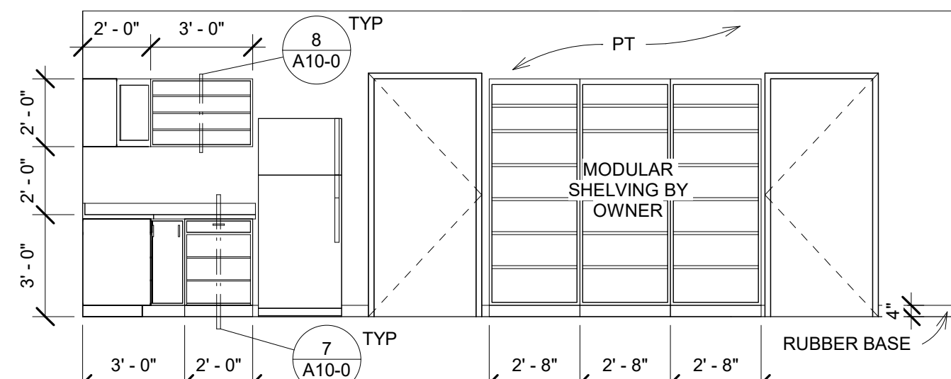
120 PHARMACY SOUTH 1/4" = 1'-0"
