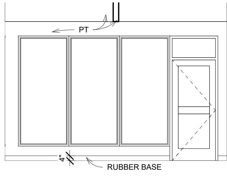
94 CONFERENCE SOUTH 1/4" = 1'-0"
