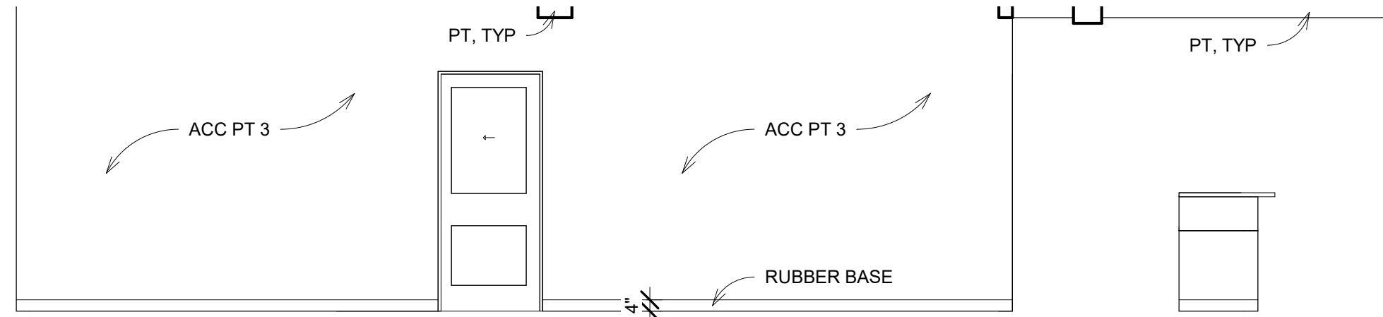
68 CORR 7 WEST 1/4" = 1'-0"
