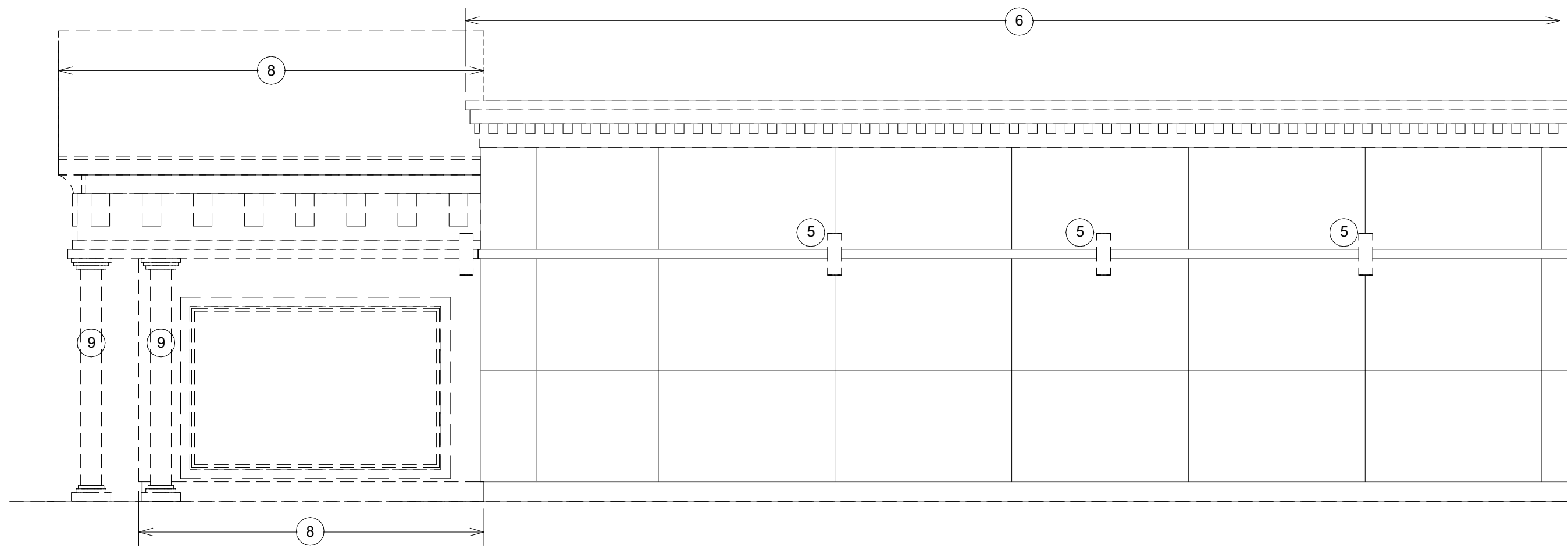
2 WEST DEMO ELEVATION - Callout 1 1/4" = 1'-0"
