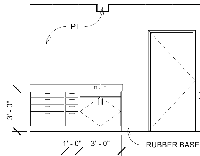
58 EXAM 6 WEST 1/4" = 1'-0"
