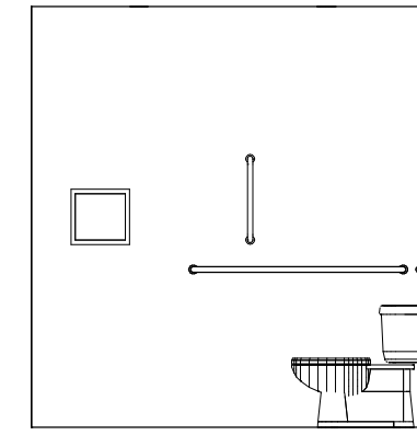
40 RR 1 WEST 1/4" = 1'-0"
